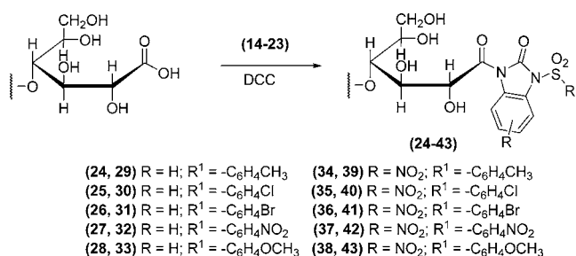
Scheme 2. Synthesis of Coupled Products ( 24–43 ) from Oxidized HES 17500 and HES 10100
