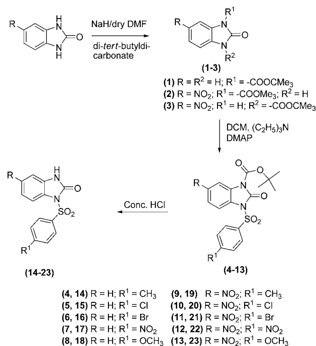
Scheme 1. Synthesis of N -Arylsulfonylbenzimidazolones (14–23)
